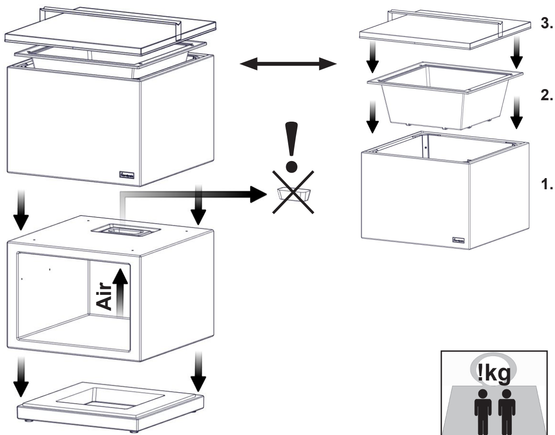
FP-AIR00-200 Air - Inside shelf for wood compartment
