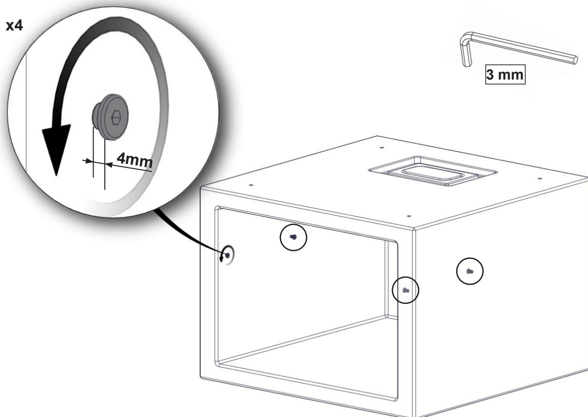
FP-AIR00-200 Air - Inside shelf for wood compartment
