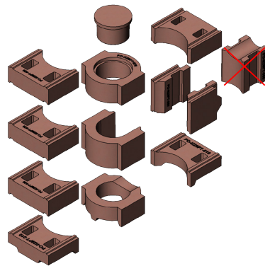
Back conection fi 150mm 124 kg
