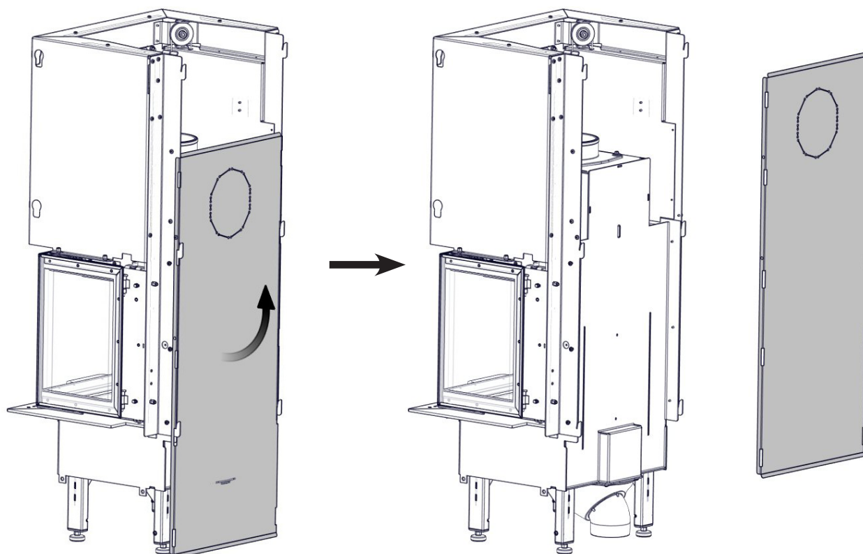
Capri_Q-24UL with ventilated chimney - optional
