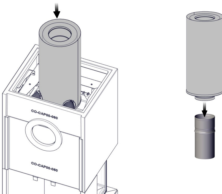
Capri_Q-24UL with ventilated chimney - optional
