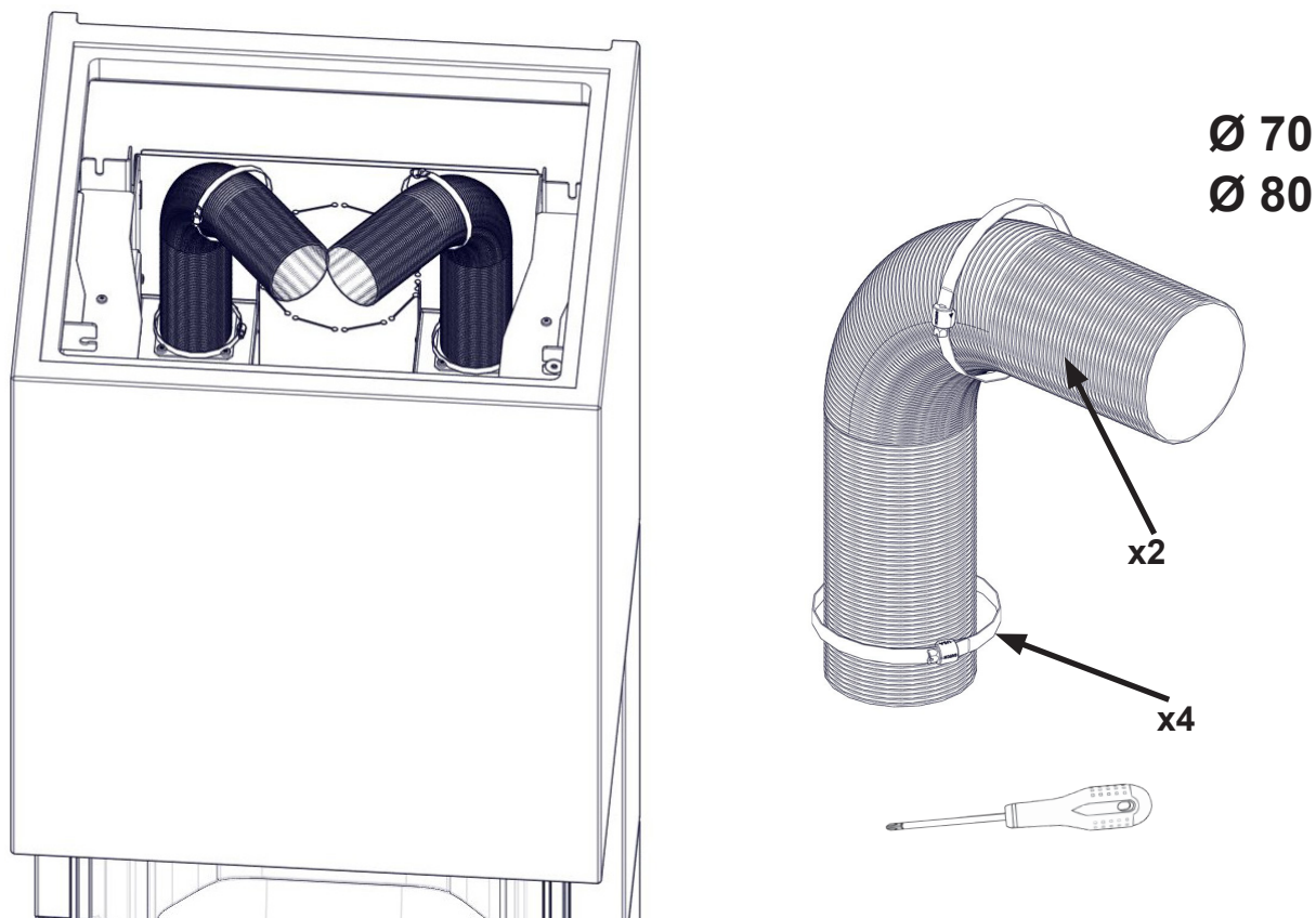
Capri_Q-24UL with ventilated chimney - optional
