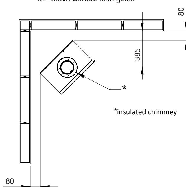
ME stove without side glass
