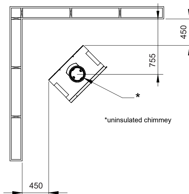
ME stove with side glass
